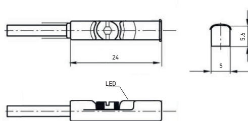
Dimensions [mm]
